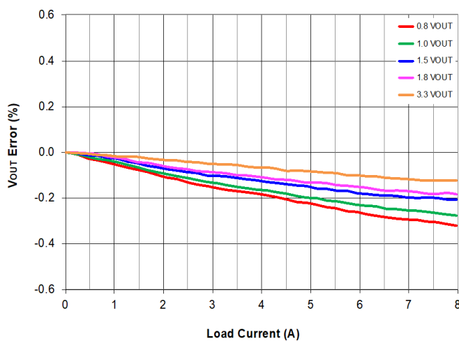
Figure 5. Load Regulation
