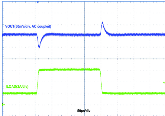
Figure 9. Load Transient, 2 A <-> 6 A, Slew Rate = 1 A/ \mu\text{s}
