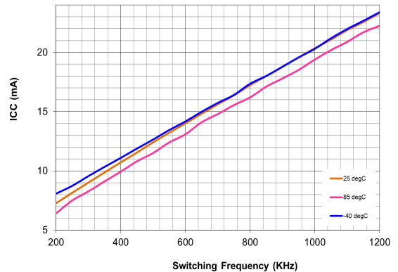
Figure 12. I_{CC} vs. Switching Frequency and Ambient Temperature
