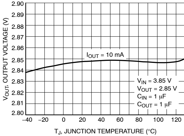
Figure 3. Output Voltage vs. Temperature – V_{OUT} = 2.85\text{ V}
