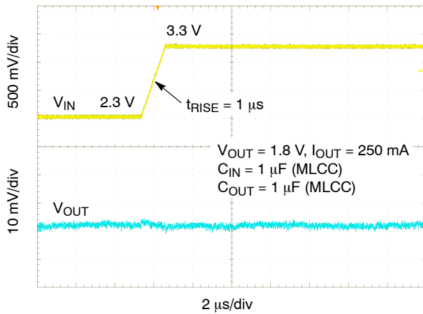
Figure 40. Line Transient Response – I_{OUT} = 250 mA
