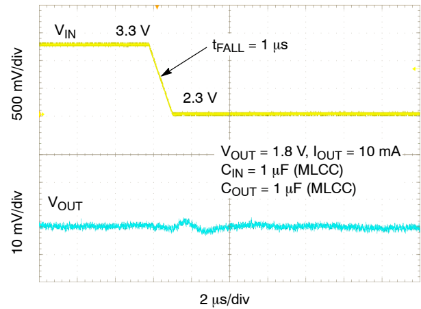
Figure 39. Line Transient Response – I_{OUT} = 10 mA
