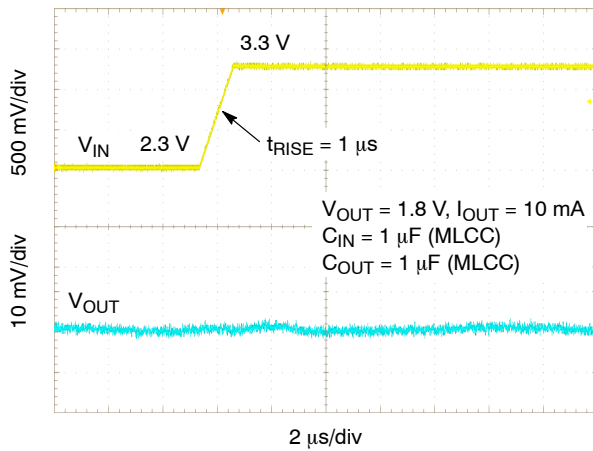
Figure 38. Line Transient Response – I_{OUT} = 10 mA
