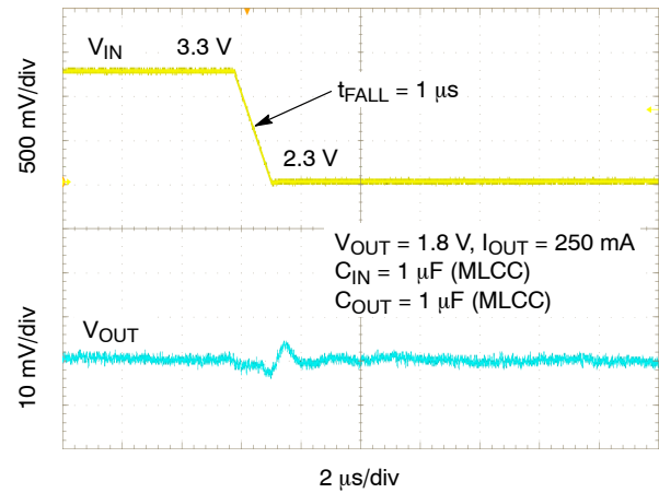
Figure 41. Line Transient Response – I_{OUT} = 250 mA
