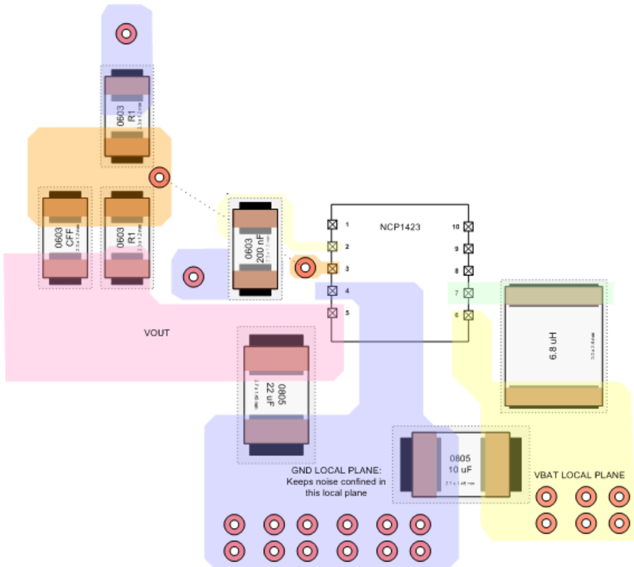
Figure 33. Layout Guidelines
