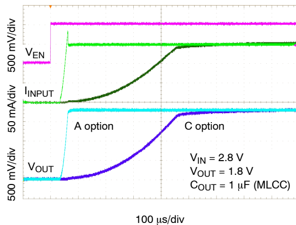
Figure 31. V_{OUT} Slew-Rate Comparison A and C option – I_{OUT} = 300 mA
