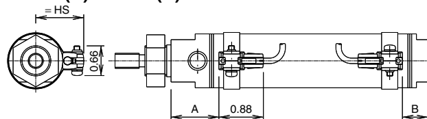
D-M9□(V)/M9□W(V)
