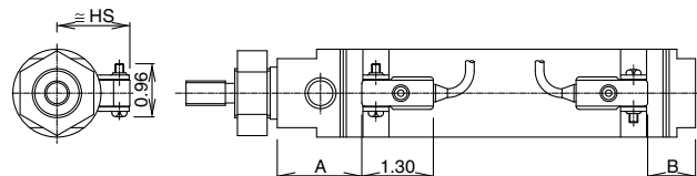
D-B5/B6/B59W
