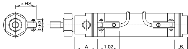
D-C7/C8
