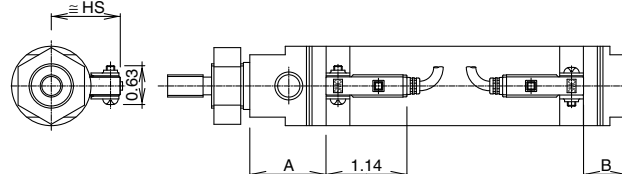
D-H7□/H7□W/H7NF/H7BAL□
