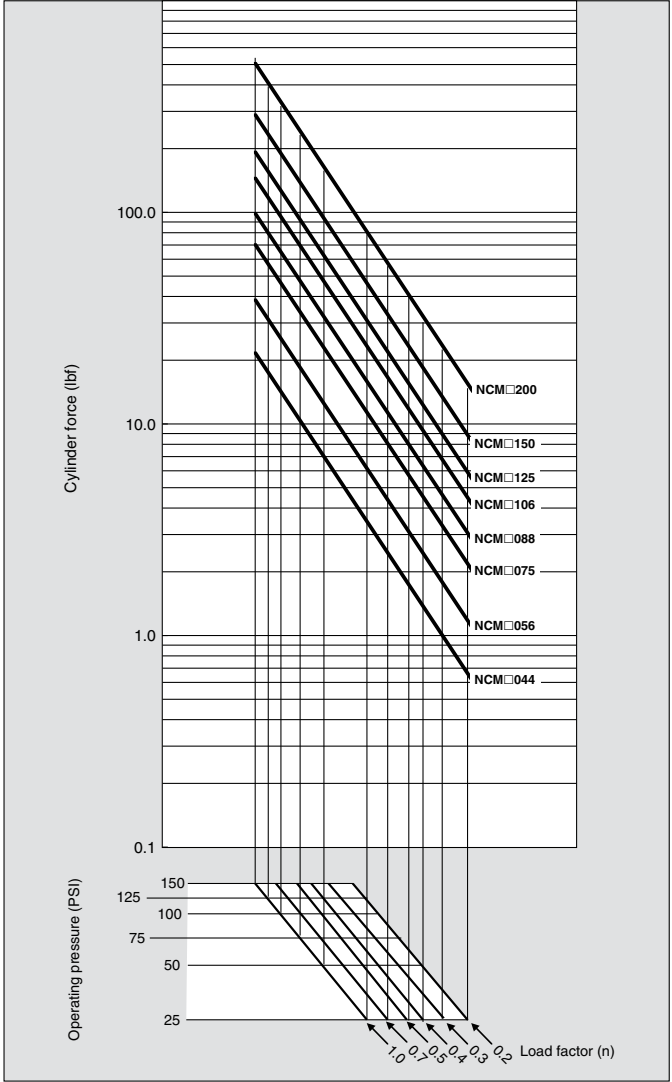
Graph (2) Retracting Side Cylinder Force (Double acting cylinder)
