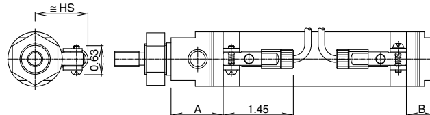
D-C73C/C80C
