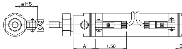
D-H7C
