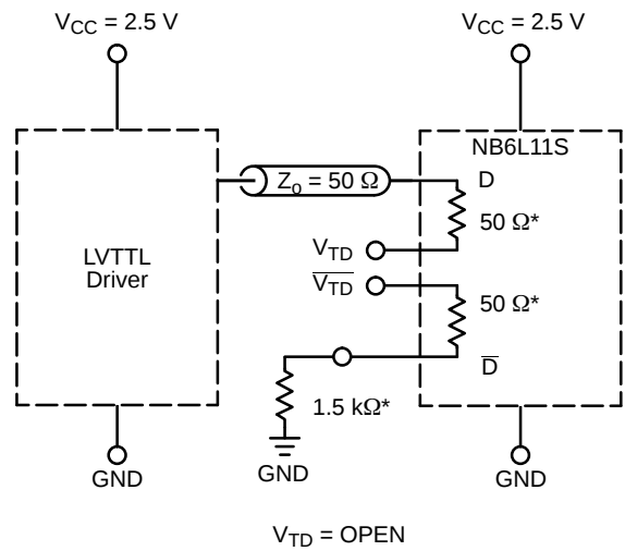
Figure 16. LVTTTL Interface
