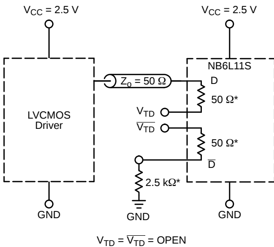
Figure 15. LVCMOS Interface
