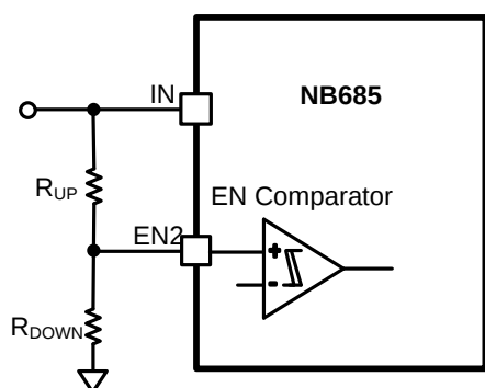
Figure 10—Adjustable UVLO
