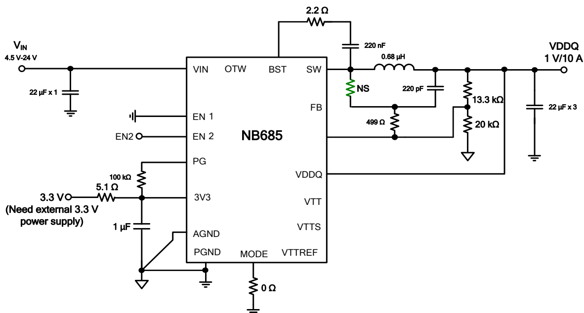
Figure 16 — Normal single buck application circuit, V_{IN} = 4.5\text{ V}-24\text{ V} , V_{OUT} = 1\text{ V} , I_{OUT} = 10\text{ A} , without V_{TT} F_s = 700\text{ kHz} .
