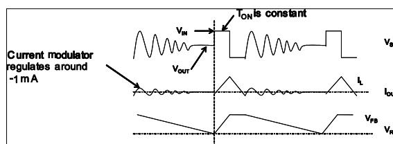
Figure 3—DCM Operation
