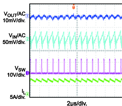
Input/Output Voltage Ripple
