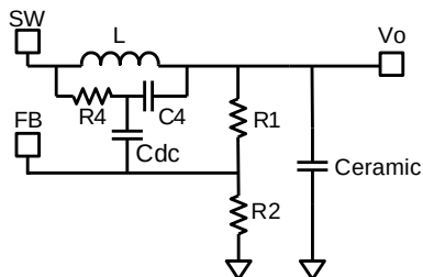
Figure 11: Simplified Circuit with Ceramic DC-Blocking Capacitor
