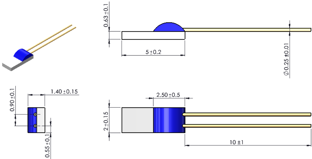
Figure 1: Mechanical dimensions of Platinum Temperature Sensor
