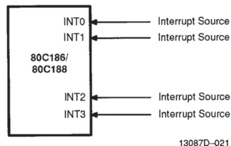
Figure 20. Fully Nested (Direct) Mode Interrupt Controller Connections
