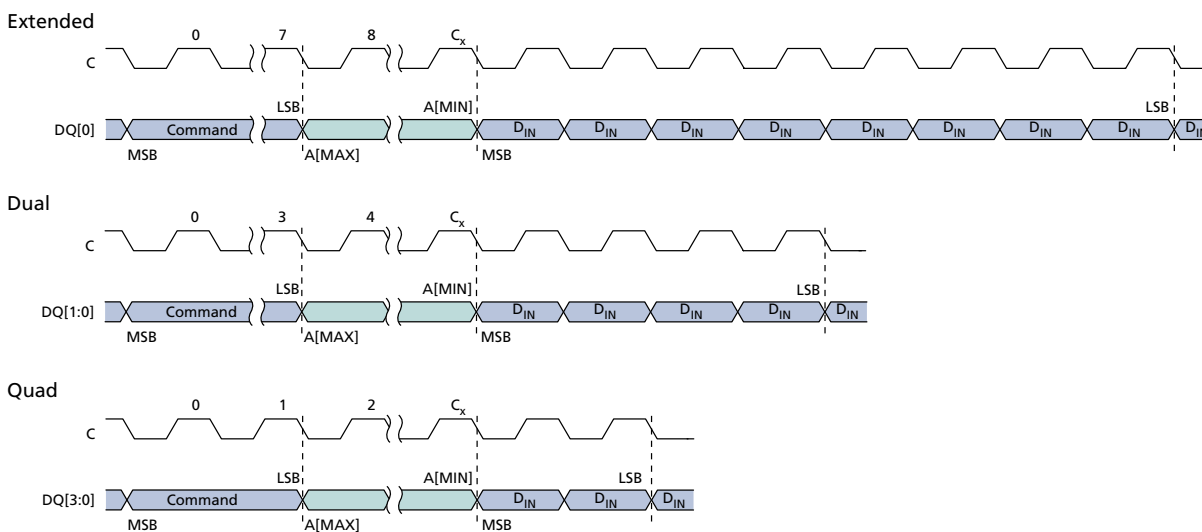
Figure 21: PAGE PROGRAM Command
