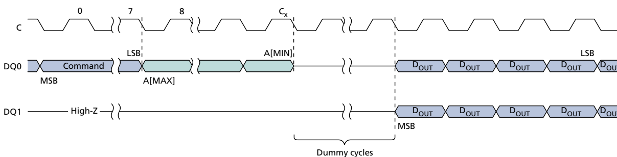
Figure 17: DUAL OUTPUT FAST READ
