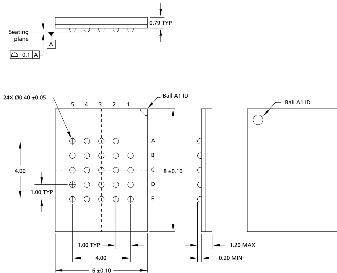
Figure 43: T-PBGA-24b05 6mm x 8mm – Package Code: 12
