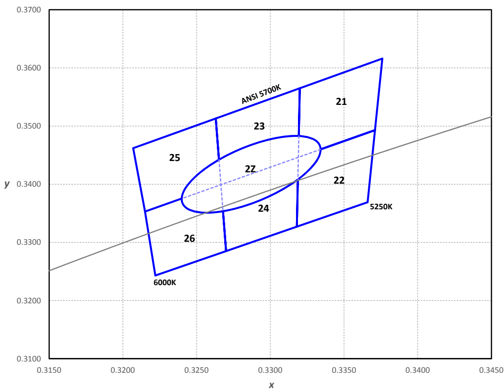
Figure 20. ANSI 5700K 1/7 th color bin structure.
