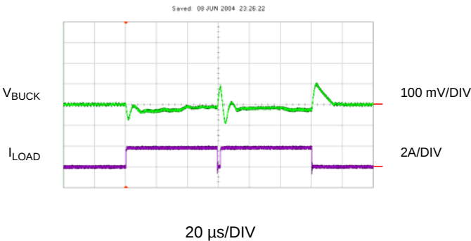
Figure 30: Double-Pulsed Load Response
