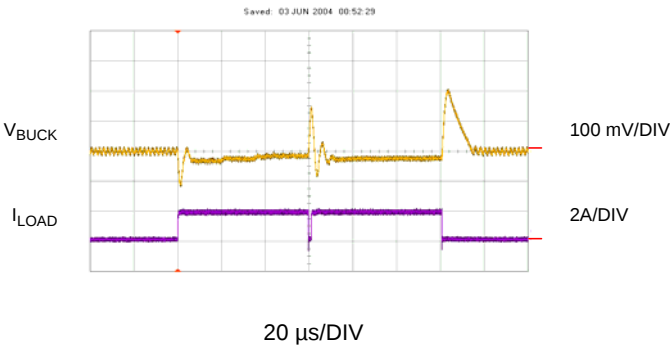
Figure 28: Double-Pulsed Load Response
