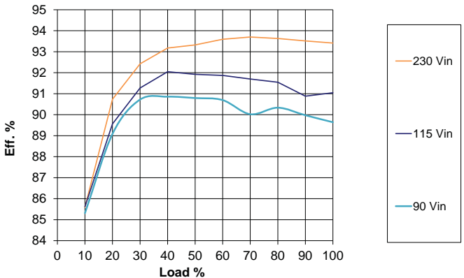
MVAC400-24 Efficiency (including 5V Aux output)
