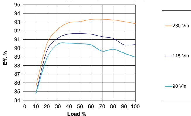
MVAC400-12 Efficiency (including 5V Aux Output)
