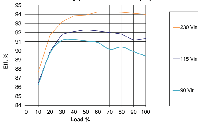
MVAC400-48 Efficiency (includes 5V Aux output)
