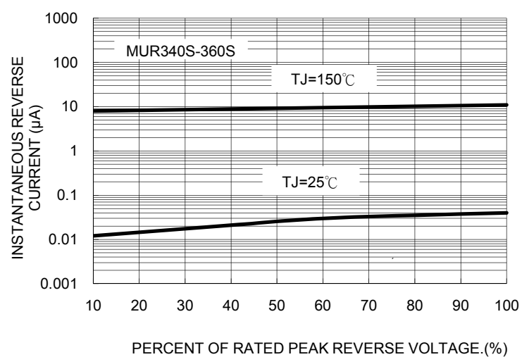
FIG. 6 TYPICAL REVERSE CHARACTERISTICS
