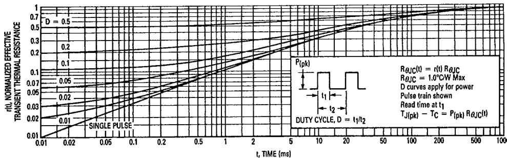
Figure 10. Thermal Response
