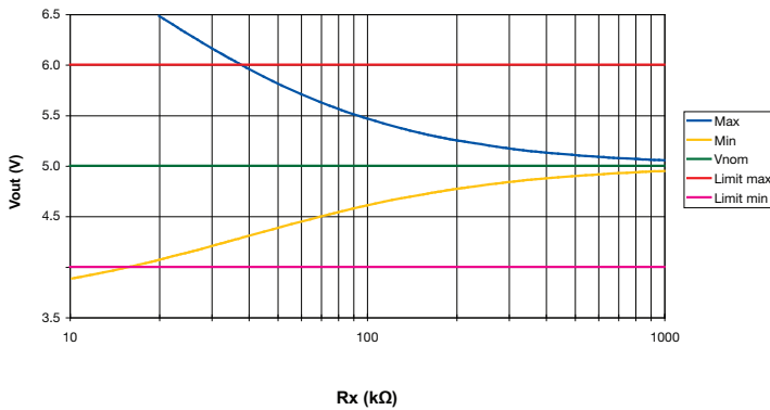
Figure 5. MTC3028S05 - Max and Min Adjustment
