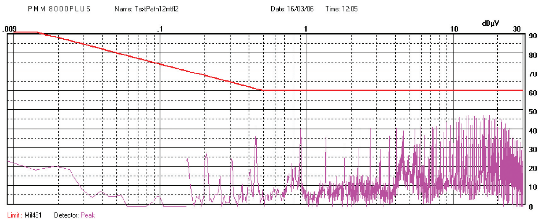
Figure 10. MTC3028S12 with MTF50 filter
