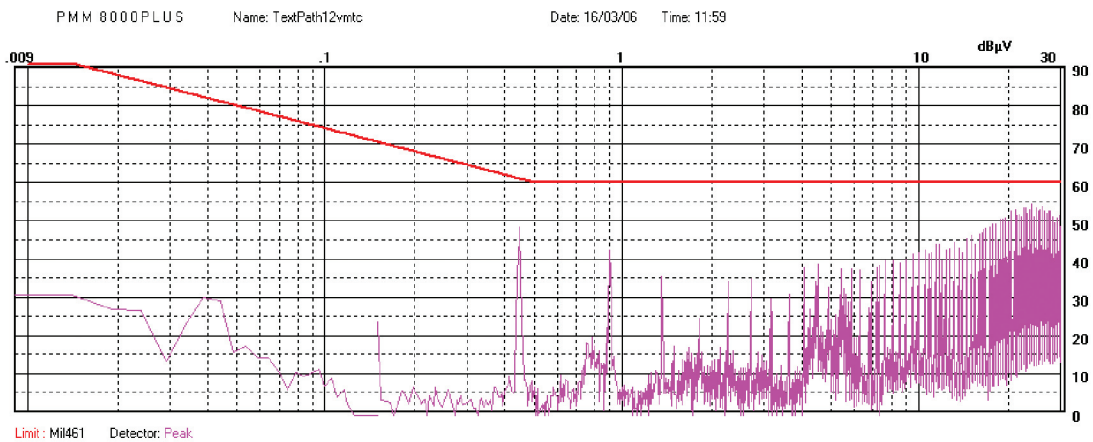
Figure 9. MTC3028S12 without a filter
