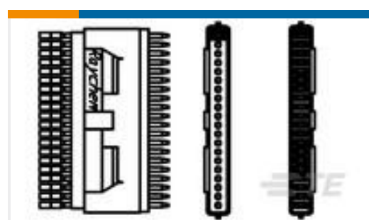
TE Part #110439-000 MTC50-YA1-016
