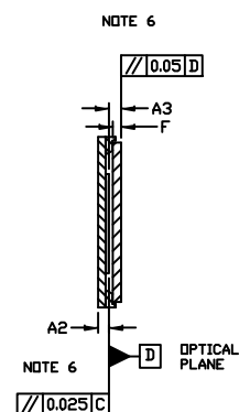
SECT. A-A
