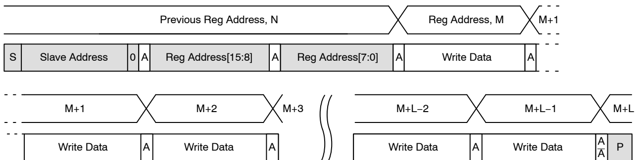
Figure 21. Sequential WRITE, Start at Random Location
