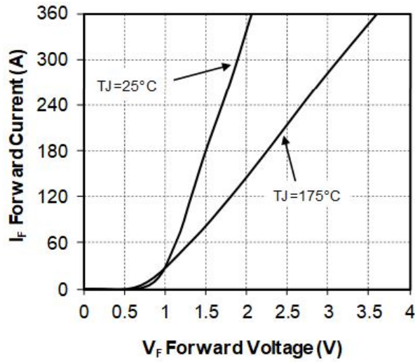
Figure 1-16. Forward Characteristics
