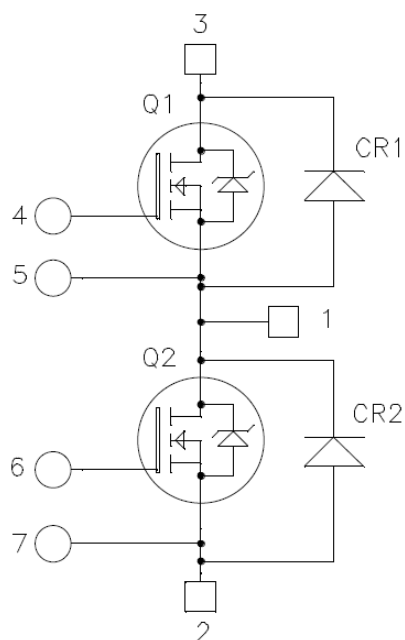
Figure 1 • MSCSM120AM042CD3AG Electrical Schematic
