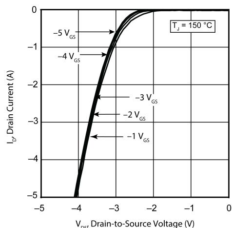
Figure 10 • I_D vs. V_{DS} 3 rd Quadrant Conduction
