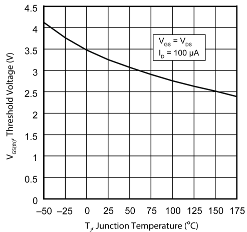
Figure 15 • Threshold Voltage vs. Junction Temp.
