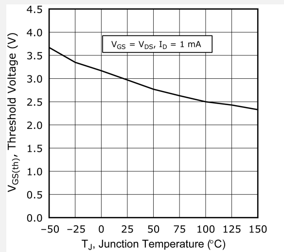
Figure 1-14. Threshold Voltage vs. Junction Temp.
