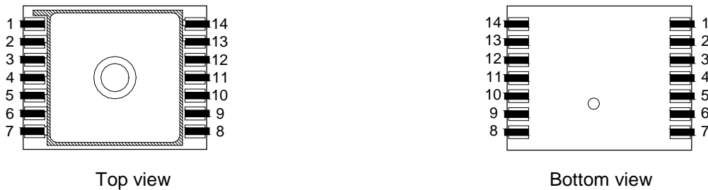
Fig. 2: Pin configuration of MS5536-CPJU, MS5536-CNJU
