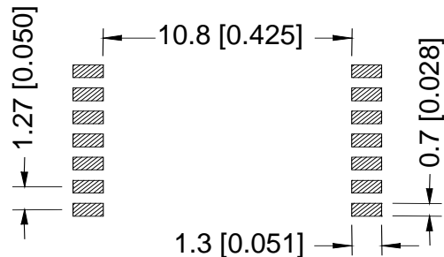
Fig. 9: Recommended pad-layout for MS5536-CPJU / MS5536-CNJU
