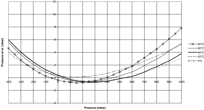
Absolute Pressure Accuracy after Calibration for MS5536-CPJU
