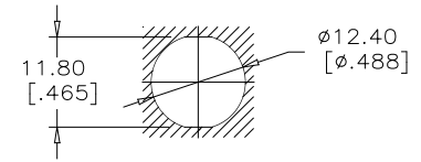
RECOMMENDED PANEL HOLE
