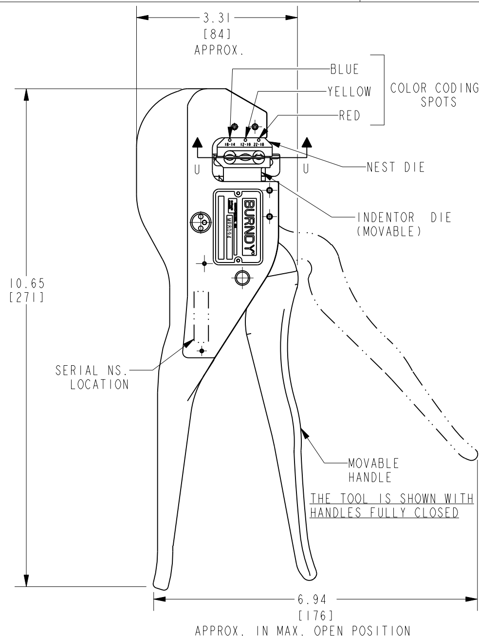
VIEW SHOWING HYTOOL WITH HANDLES FULLY OPENED
