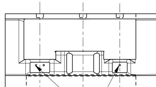
VIEW U-U SYMBOLS ARE IMPRESSED ON NYLON OF INSULUGS. (AS SHOWN)
