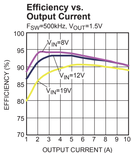
Figure 31 — Efficiency Curve
