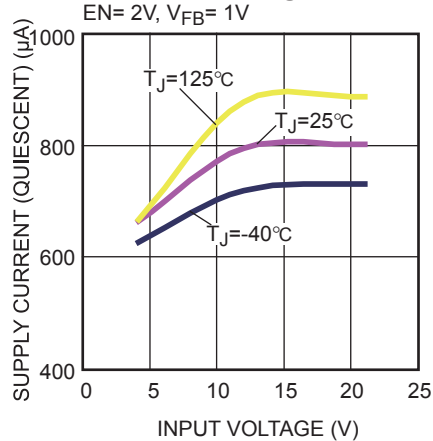
Supply Current (Quiescent) vs. Input Voltage
