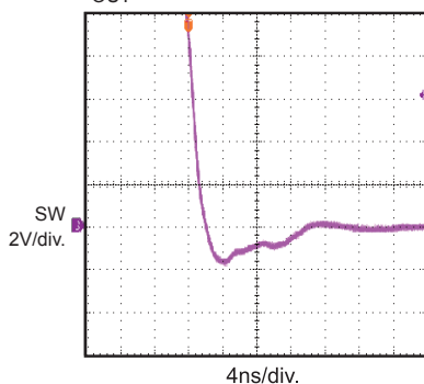
Dead Time (off) I_{OUT} = 10A
