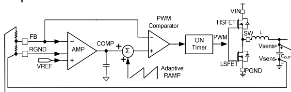
Figure 2: COT Control
