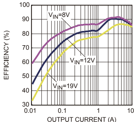
Figure 22 — Efficiency Curve
