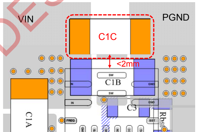
Figure 16—PCB LAYOUT
