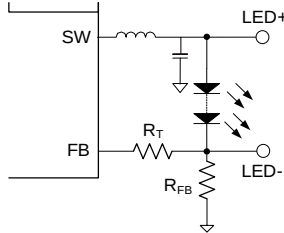
Figure 5: Feedback Network
