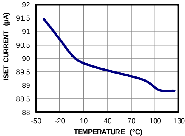
ISSET Current vs. Temperature High-side source current, I_{OUT} = 1A
