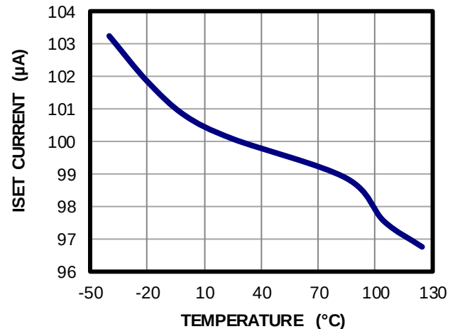
ISSET Current vs. Temperature High-side sink current, I_{OUT} = 1A
