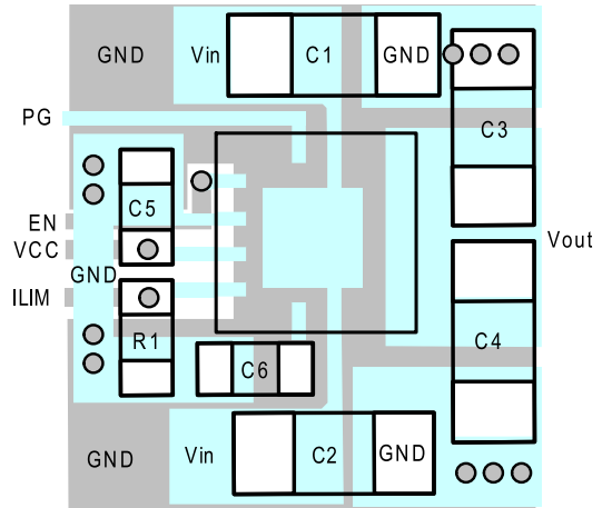
Figure 5: Recommended Layout
