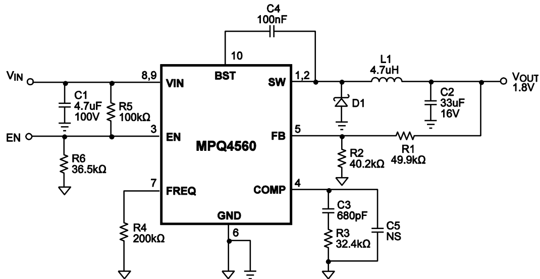
Figure 3: Typical Application, 1.8V Output
