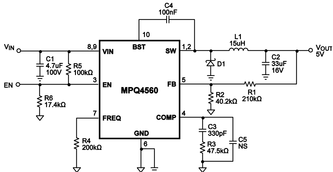
Figure 4: Typical Application, 5V Output
