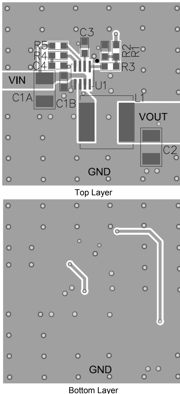
Figure 7: Recommended PCB Layout
