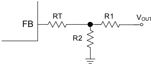
Figure 4: T-Type Network
