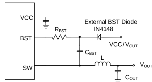
Figure 9: Optional External Bootstrap Diode to Enhance Efficiency
