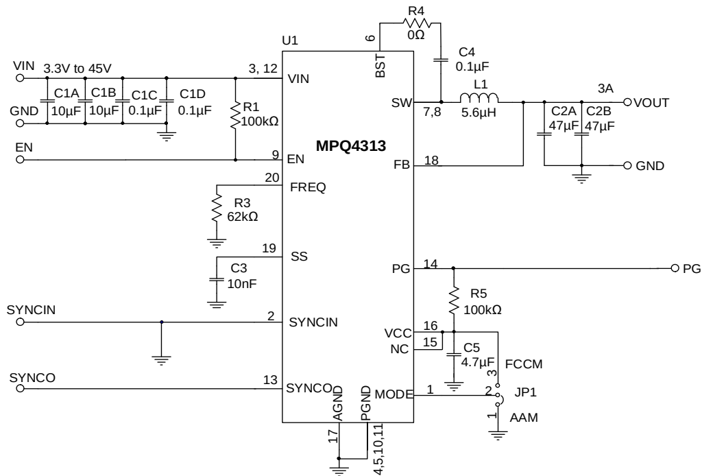
Figure 14: f_{sw} = 470kHz , Fixed Output
