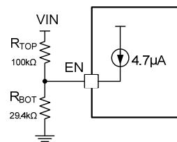
Figure 5: V IN UVLO Program
