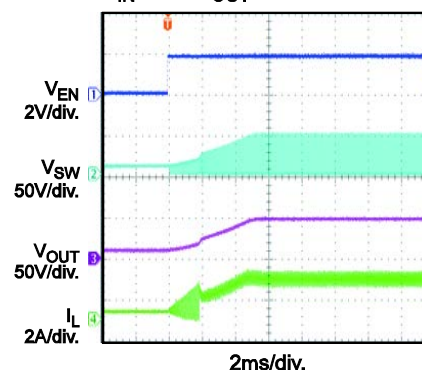
EN Start-Up V_{IN} = 10V , I_{OUT} = 0.4A
