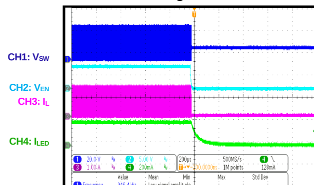
Shutdown through EN/DIM
