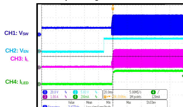
Start-Up through EN/DIM
