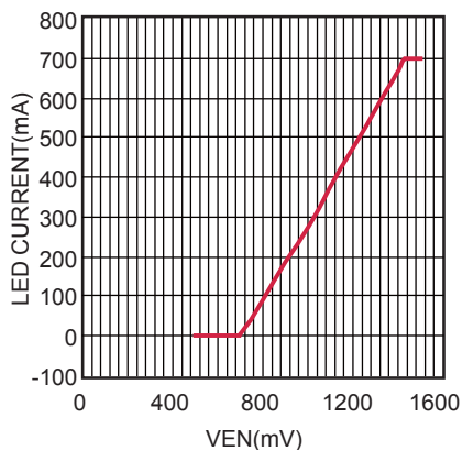
LED Current vs. VEN
