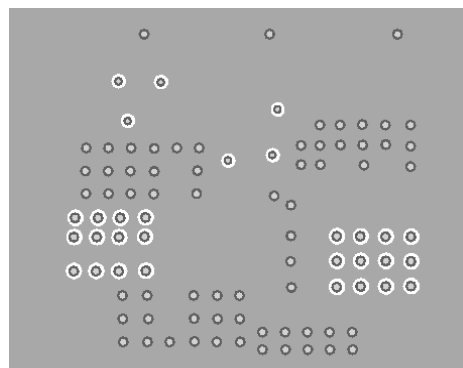
Mid-Layer 1
