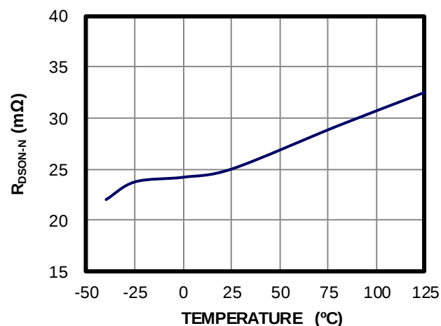
Low-Side Switch On Resistance vs. Temperature
