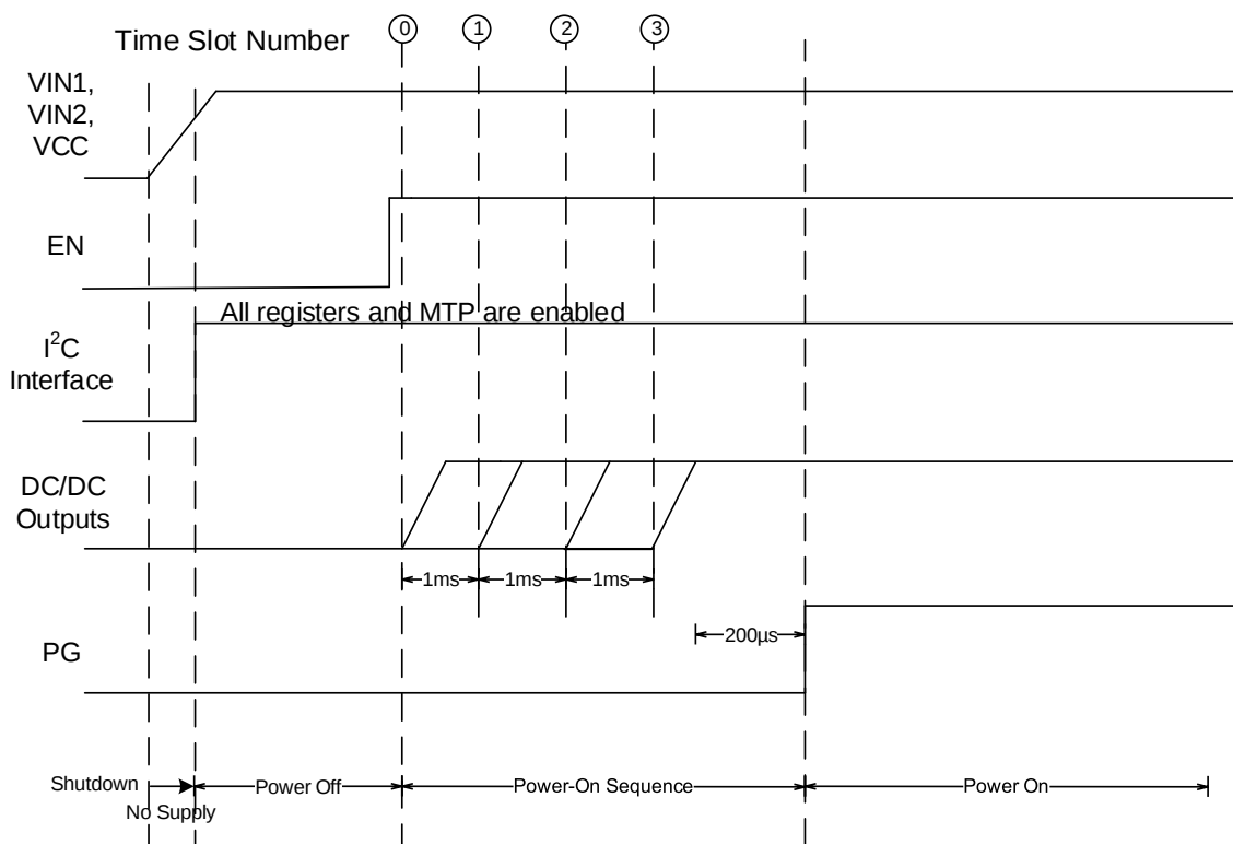
Figure 7: Power-On Sequence
