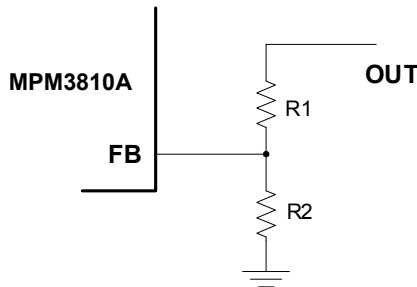
Figure 2: Feedback Network
