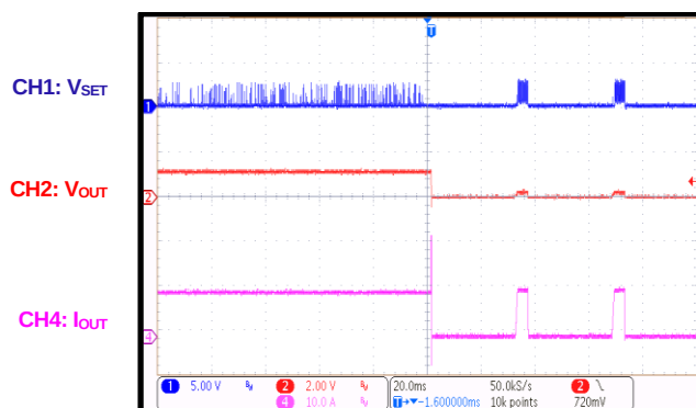
Short-Circuit Protection
