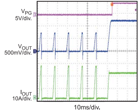
Over Current Protection Recovery
