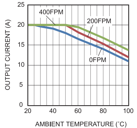
Output Current De-Rating 12V to 5V, 600kHz
