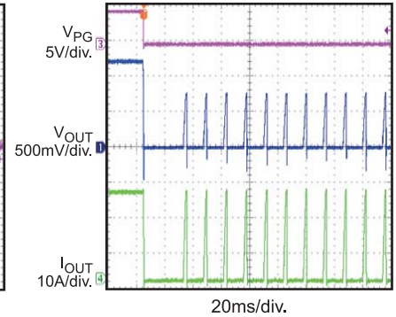
Over Current Protection (OCP)
